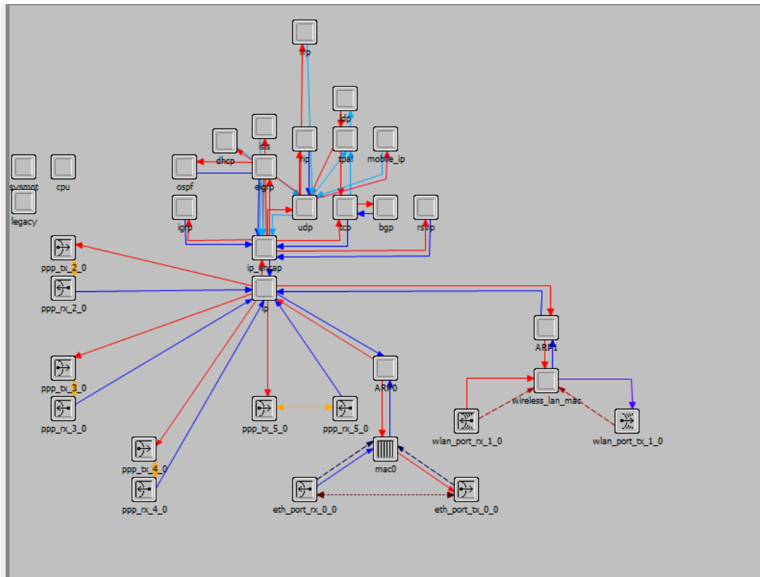
Figure 4.1: WLAN access point node model
